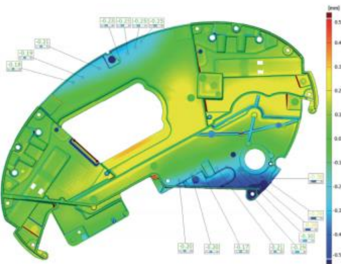
Figure 30: Optical 3D displacement and deformation measurement
