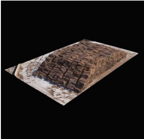
Fig. 7 – Volumetric Measurements by UAV
