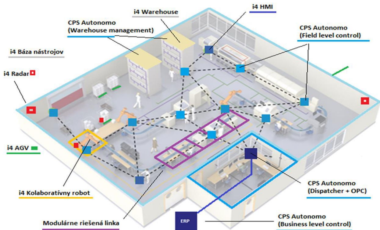
Fig. 10 – SMART Factory - TIA
