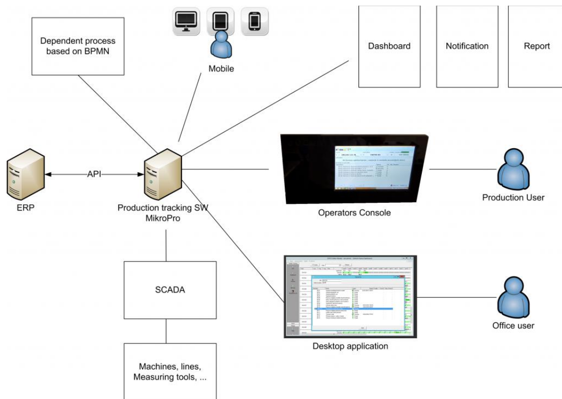
Figure: Scheme of the system mpPTS
