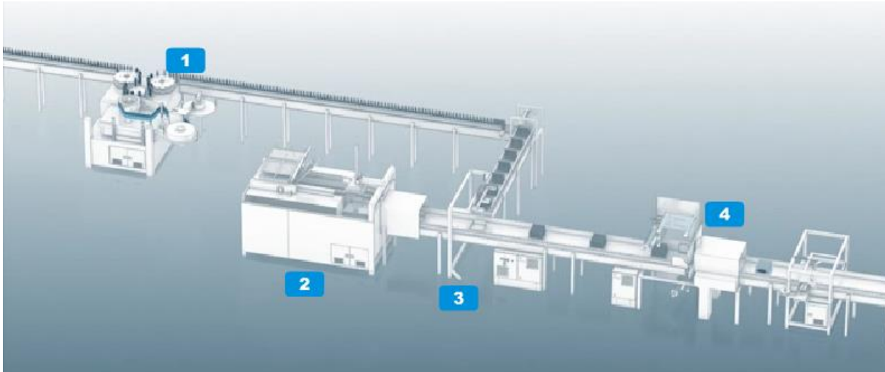
Figure 6 FESTO secondary packaging
