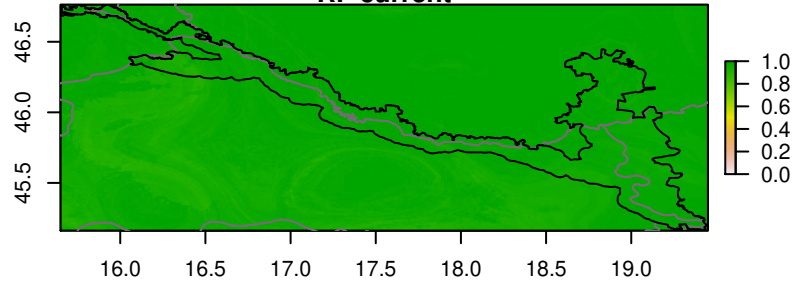
RF current
