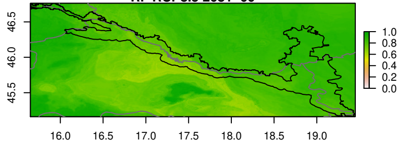
RF RCP8.5 2081-00
