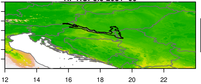
RF RCP8.5 2081-00
