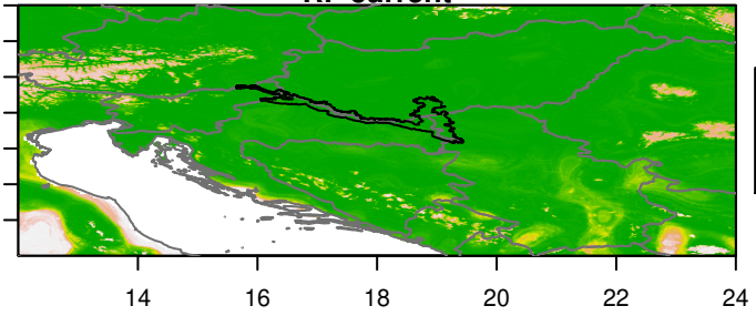
RF current
